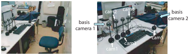
Figure 7. Camera configuration.
