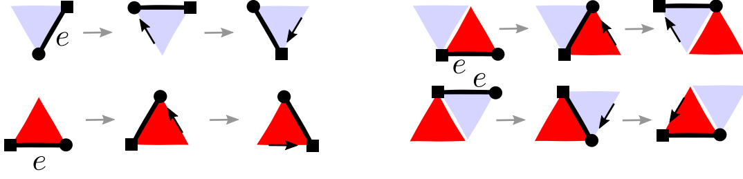
Figure 15: (Left) The second flip of the edge e does not counteract the first flip of e . (Right) The second flip of e counteracts the first one.
