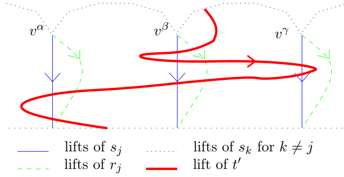
Figure 8: A view of \tilde{\mathcal{M}}(s, j, \tilde{t}') , the lifts of r_j , s_j , and the lift \tilde{t}' . Here, [r + s/t'] = \bar{r}_j^\beta \bar{s}_j^\beta s_j^\beta r_j^\beta s_j^\gamma \bar{s}_j^\gamma \bar{r}_j^\beta \bar{s}_j^\beta \bar{r}_j^\alpha \bar{s}_j^\alpha s_j^\alpha r_j^\alpha .
